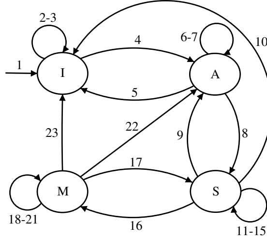
Fig. 1. OLSR Extended Finite State Machine (see Appendix for details)
